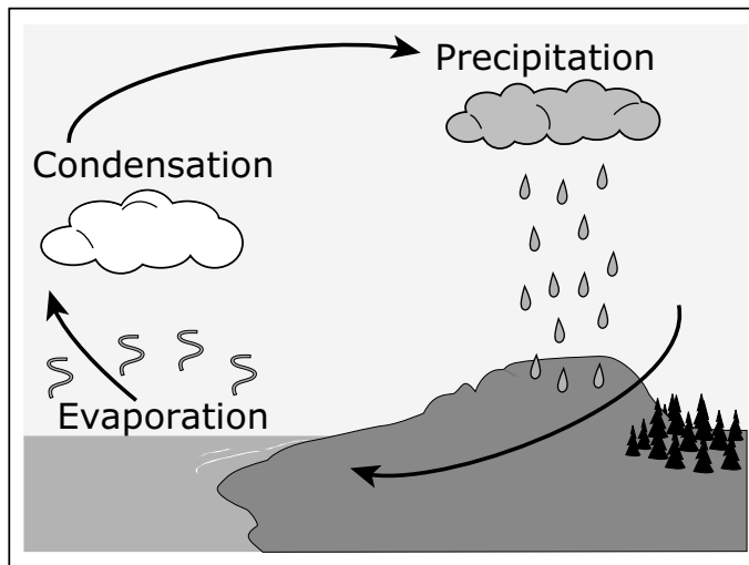
Water Cycle
